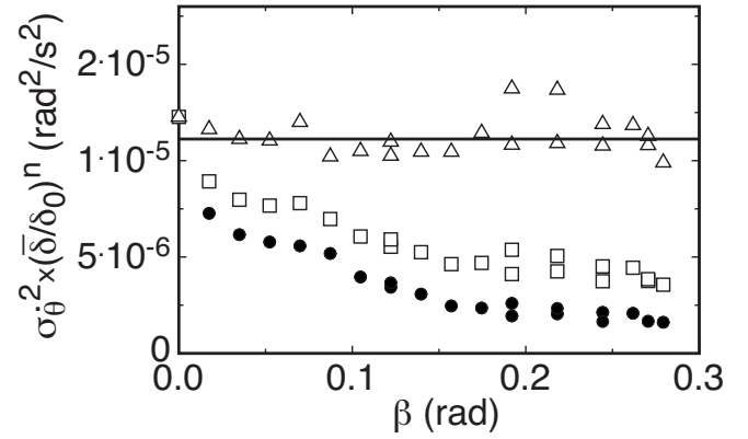
FIG. 5. The variance of rotation rate \sigma_\theta^2 \times (\bar{\delta}/\delta_0)^n as a function of tilt angles \beta at R = 2.8 \times 10^8 . The variance is multiplied by (\bar{\delta}/\delta_0)^n with several different values of n . Solid circles: n=0 , i.e., the bare variance \sigma_\theta^2 . Open squares: n=1 , which is predicted by the model in the linear approximation to yield a constant independent of \beta . Open triangles: n=2.29 , where n is obtained from a best fit of a horizontal line to the data.
