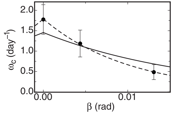
FIG. 4. The rate of cessations \omega_c as a function of tilt angle at R=1.1 \times 10^{10} . Solid line: a fit of \omega_c \propto \exp(-2\delta_0\delta_\beta\beta/D_\delta) to the data with D_\delta/(2\delta_0\delta_\beta) fixed at the value 0.017 based on measurements at \beta=0 . Dashed line: a similar fit with D_\delta/(2\delta_0\delta_\beta)=0.010 least-squared adjusted.
